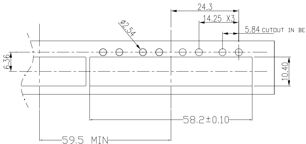
RECOMMENDED BEZEL CUT-OUT SINGLE SIDED APPLICATIONS
