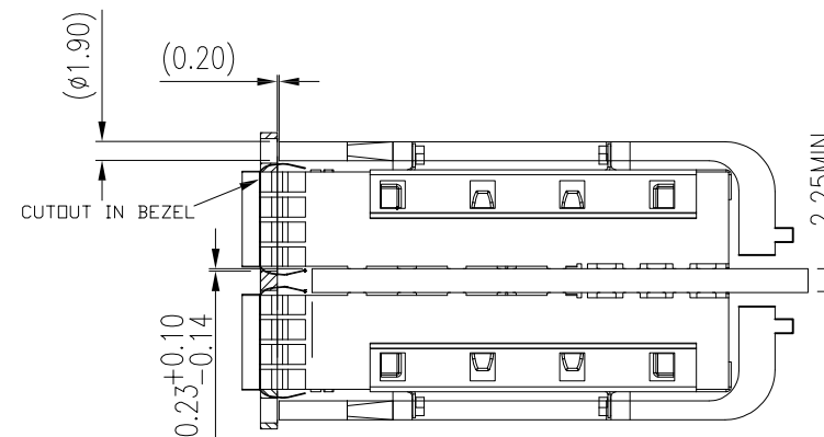
MOUNTED BELLY TO BELLY PC BOARD SHOWN THRU RECOMMEND BEZEL
