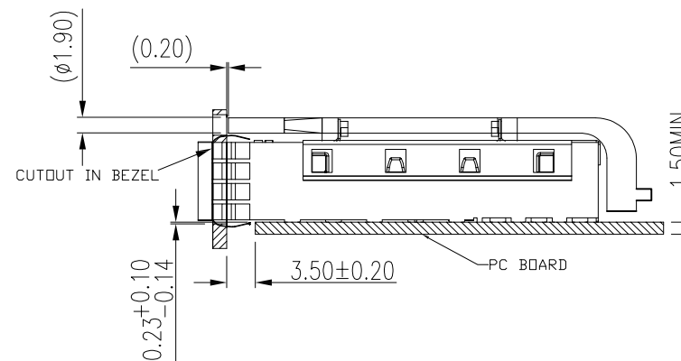
MOUNTED ON PC BOARD SHOWN THRU RECOMMEND BEZEL
