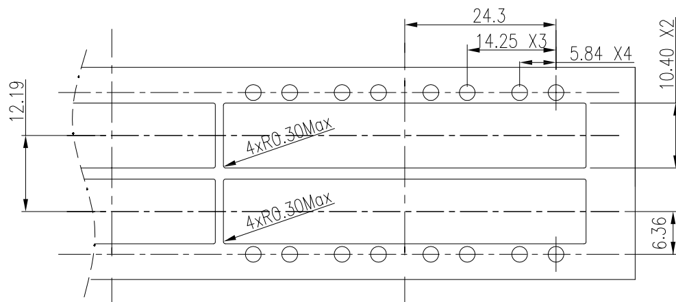
RECOMMENDED BEZEL CUT-OUT BELLY TO BELLY APPLICATIONS
